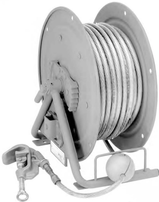
型號SGCR 10-17-19彈簧捲取 Model SGCR 10-17-19 Spring Rewind
