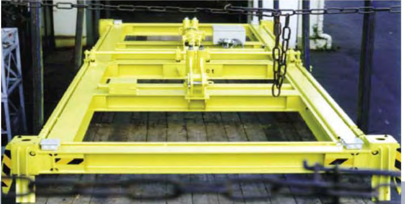
Container spreaders with central bolting
