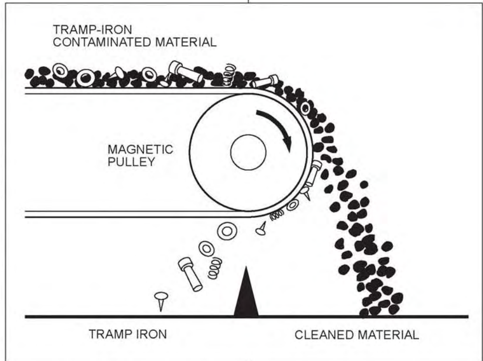
Figure 1. Operating Principle of a Magnetic Pulley
